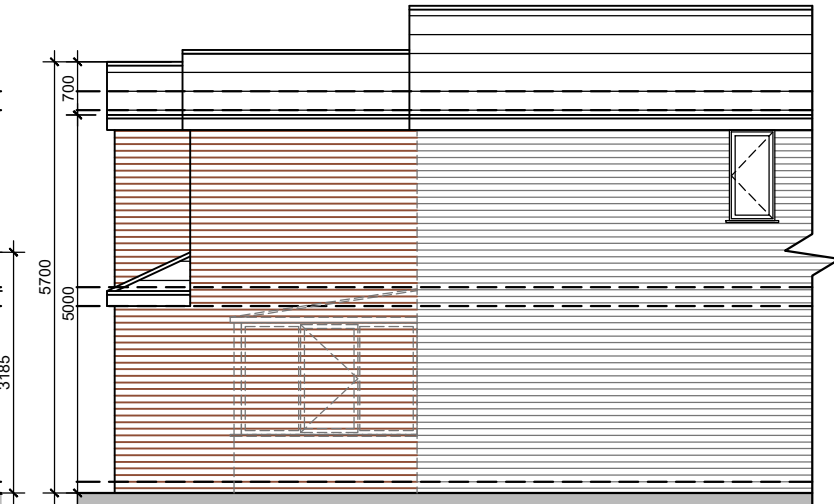
SIDE ELEVATION 1:100
