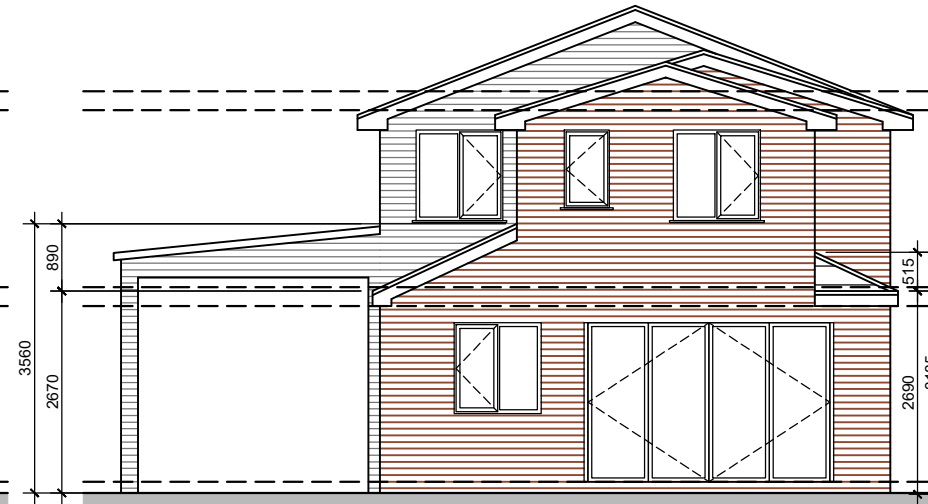
REAR ELEVATION 1:100
